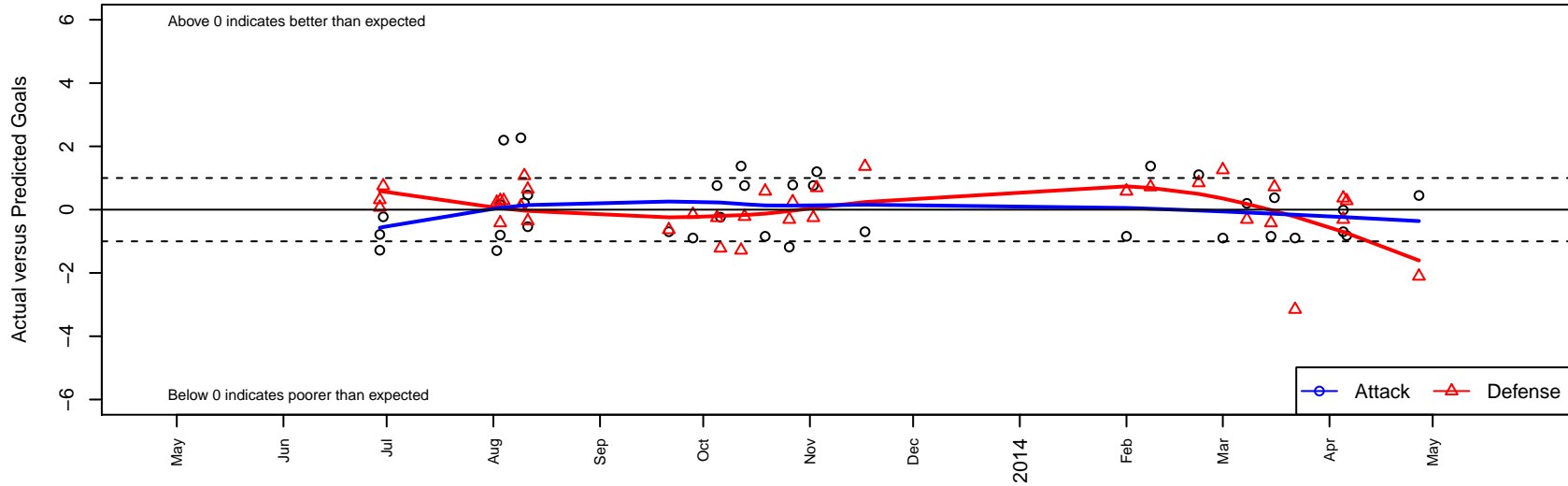
Kitsap Pumas G00 Dots are actual minus expected GF (blue circles) and GA (red triangles). Blue line is smoothed change in attack strength. Red is smoothed change in defense strength.
